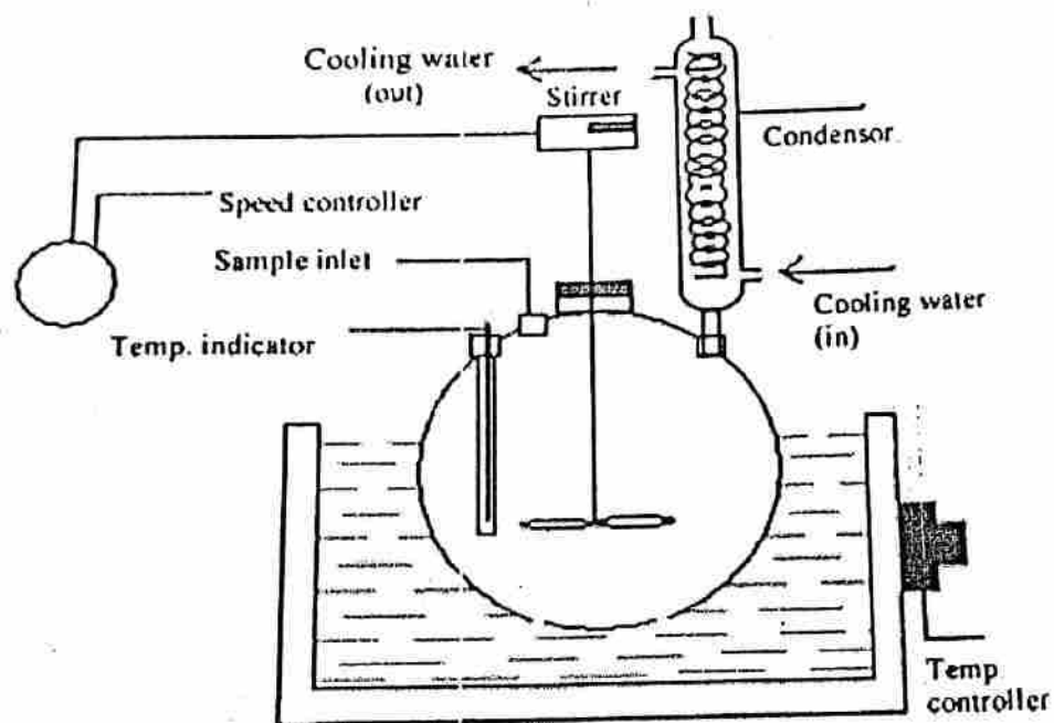
Fig. 1 Sketch of transesterification process setup
