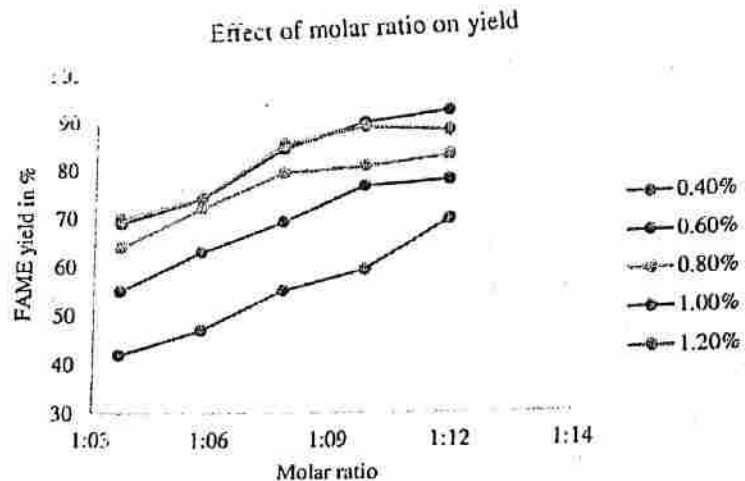
Fig. 3 Comparison of variation of Molar Ratio for different catalyst percentages
