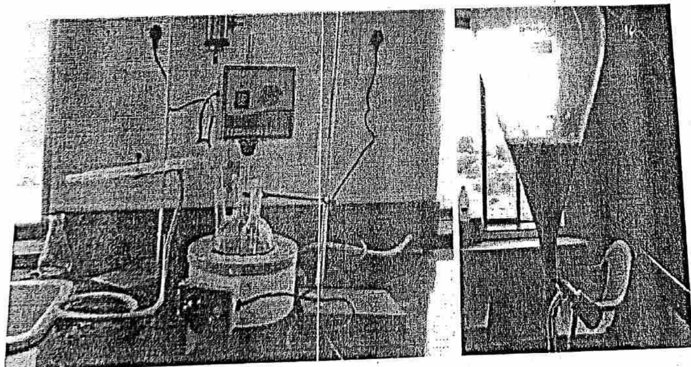
Fig. 1 Sketch of transesterification process setup
